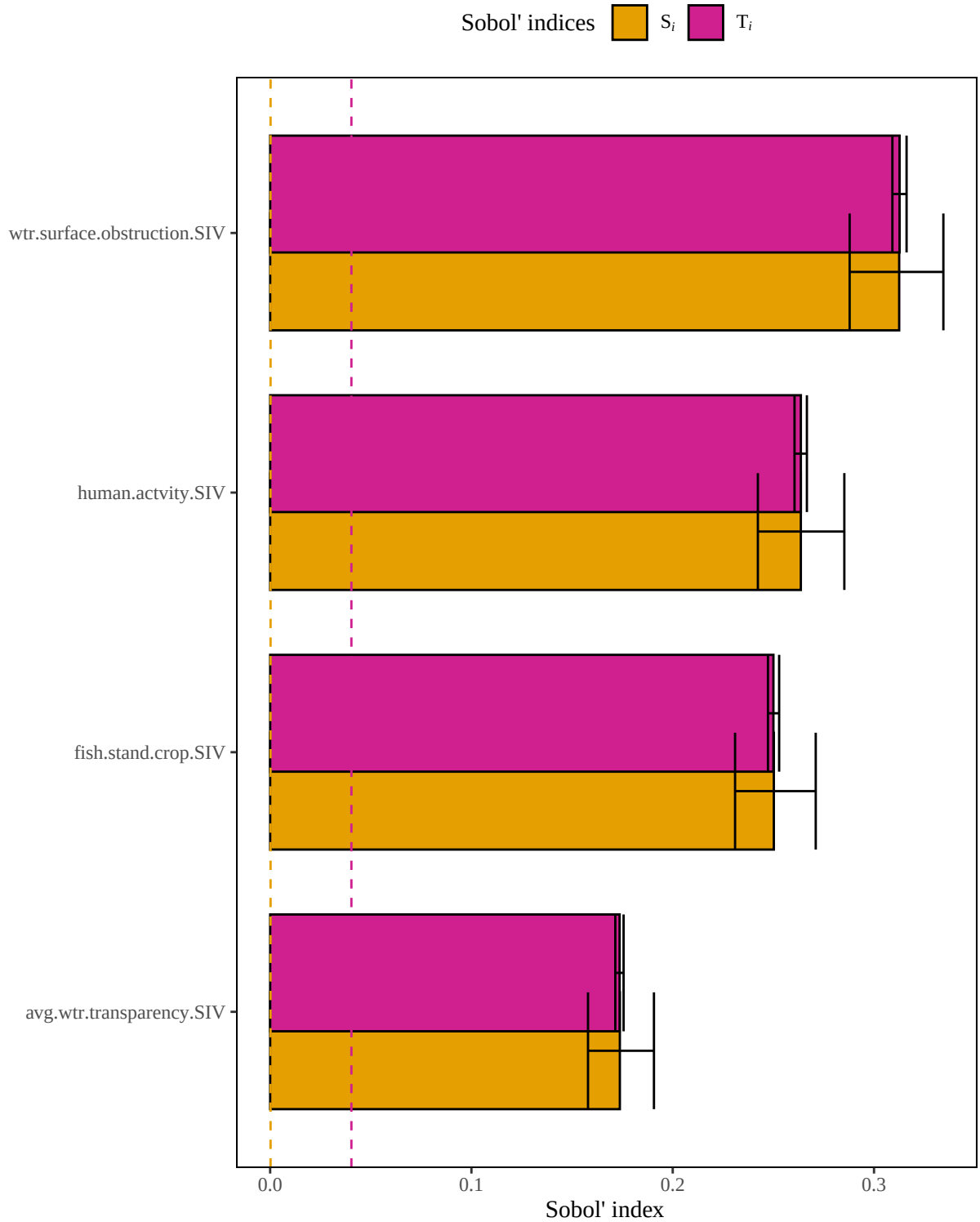
Figure 4. Results of a sensitivity analysis for the ospreyLac model based on an arithmetic mean structure. Dashed lines represent baseline numerical approximation error for S_i and T_i ( i.e. , dummy variables).
