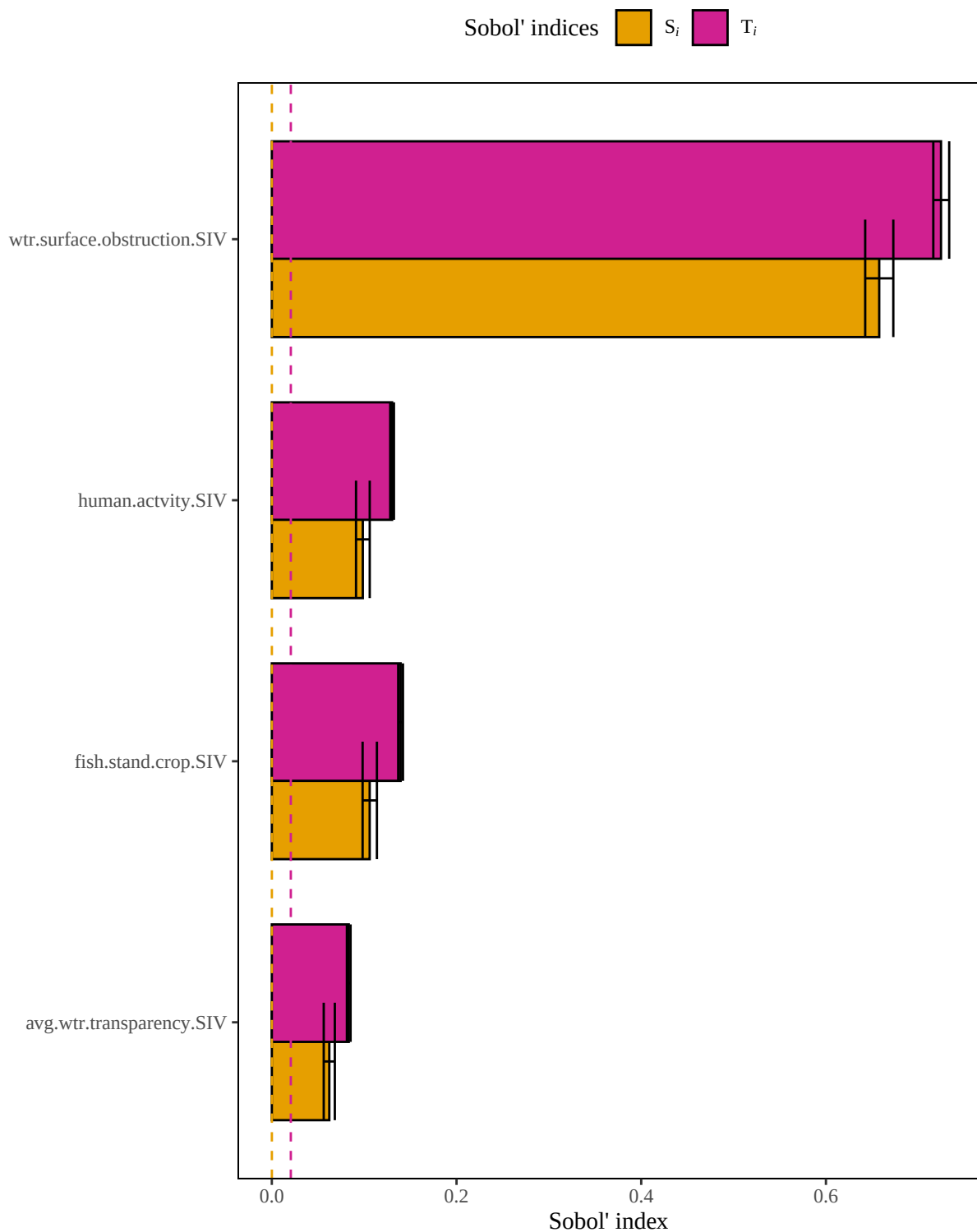
Figure 5. Results of a sensitivity analysis for the ospreyLac model based on a geometric mean structure. Dashed lines represent baseline numerical approximation error for S_i and T_i ( i.e. , dummy variables).
